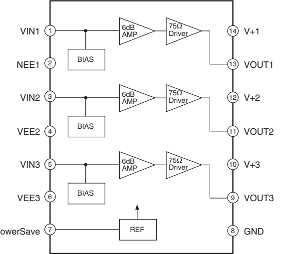
IC853: NJM2581M Video Amp
