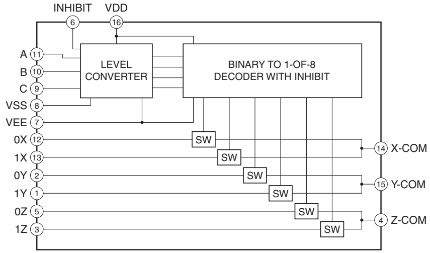
IC851, 852: TC74HC4053AF Analog Multiplexer/Demultiplexer
