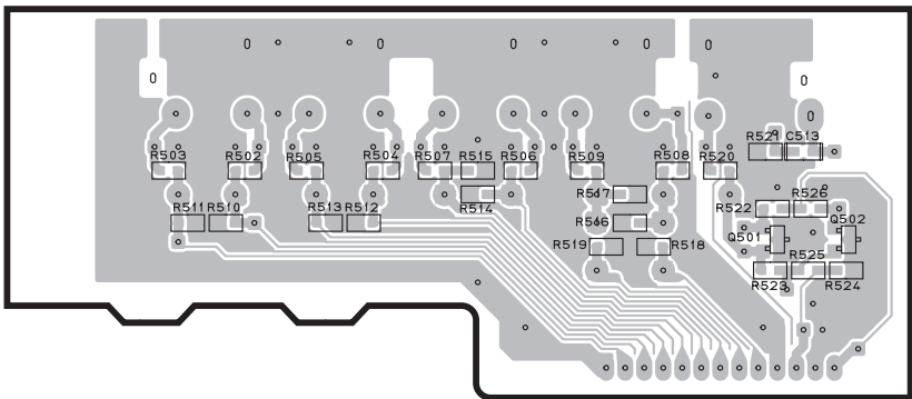
FUNCTION (2) P. C. B. (Surface Mount Device)
