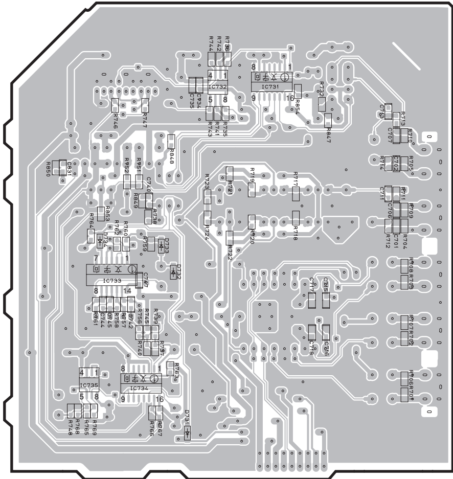
FUNCTION (5) P. C. B. (Surface Mount Device)
