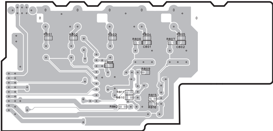
FUNCTION (6) P. C. B. (Surface Mount Device)
