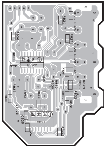
FUNCTION (7) P. C. B. (Surface Mount Device)
